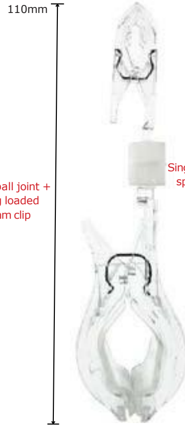
Clear Pop Clip - 110mm H TC35-1C
